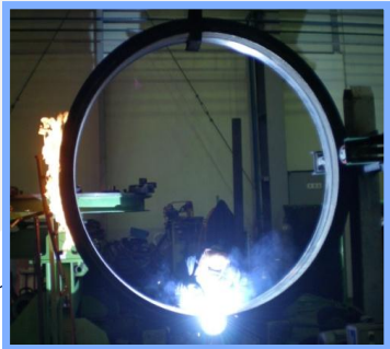
Weld Overlay
